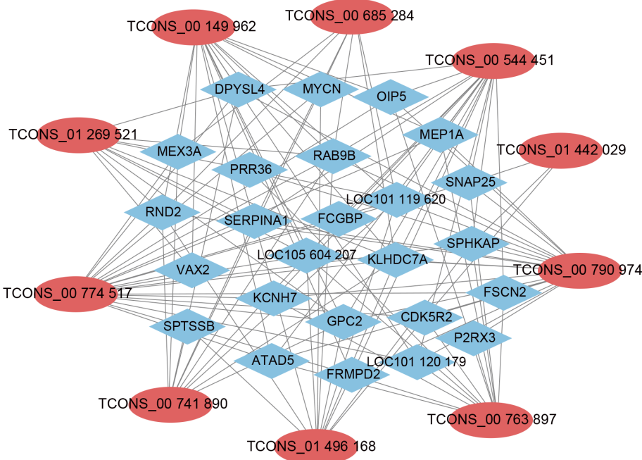
Figure 4 Co-expression network of lncRNAs and their potentially regulated genes. Red nodes represent lncRNAs, blue nodes represent their potentially regulated genes.
