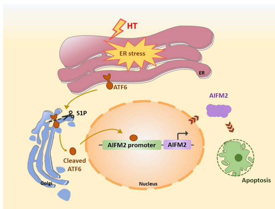
Figure 7 Mechanistic representation of ATF6-mediated exacerbation of apoptosis in early porcine embryonic development through regulation of organelle homeostasis under HT conditions
