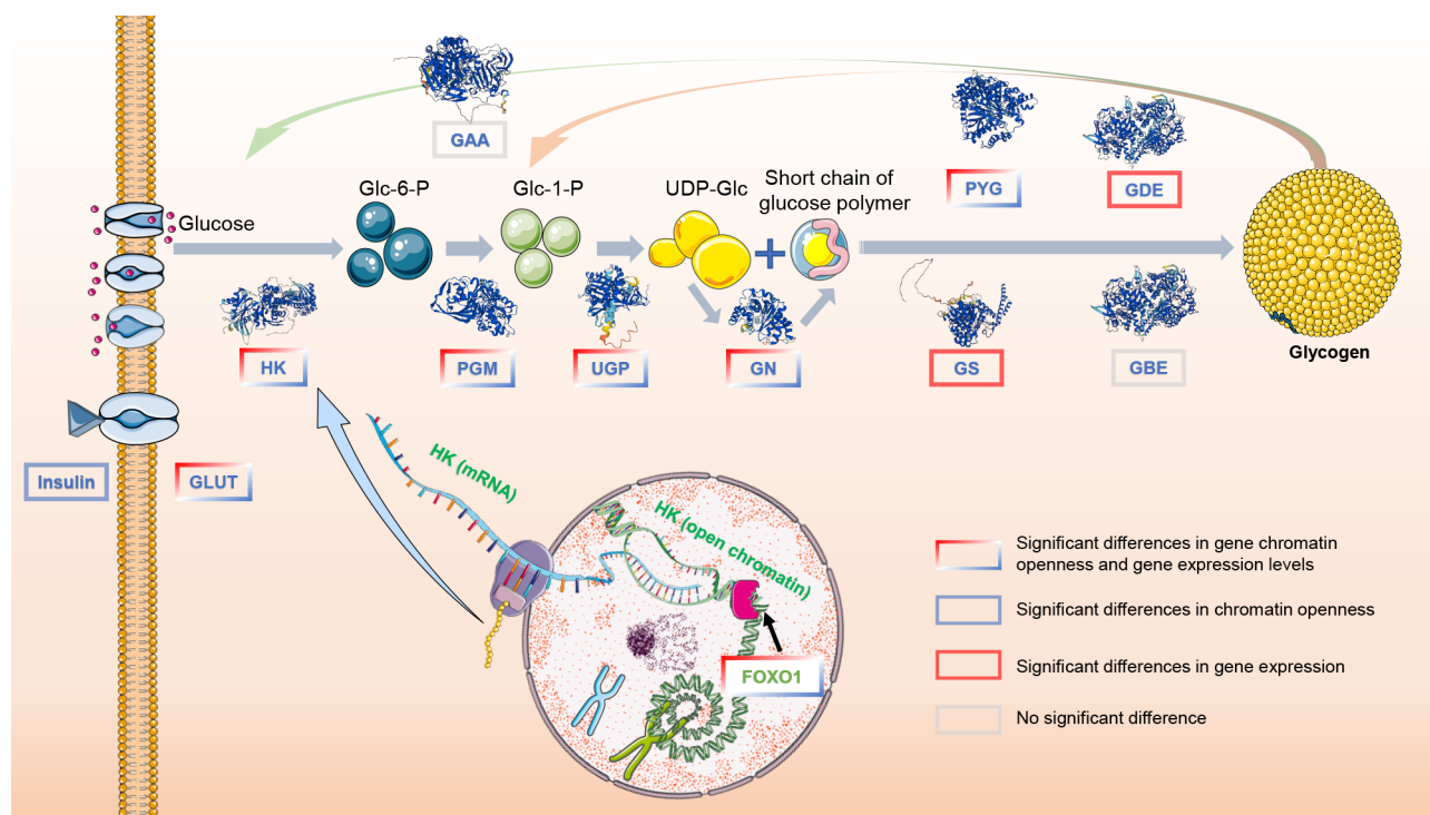
Figure 8 Diagram of glycogen metabolism pathway
