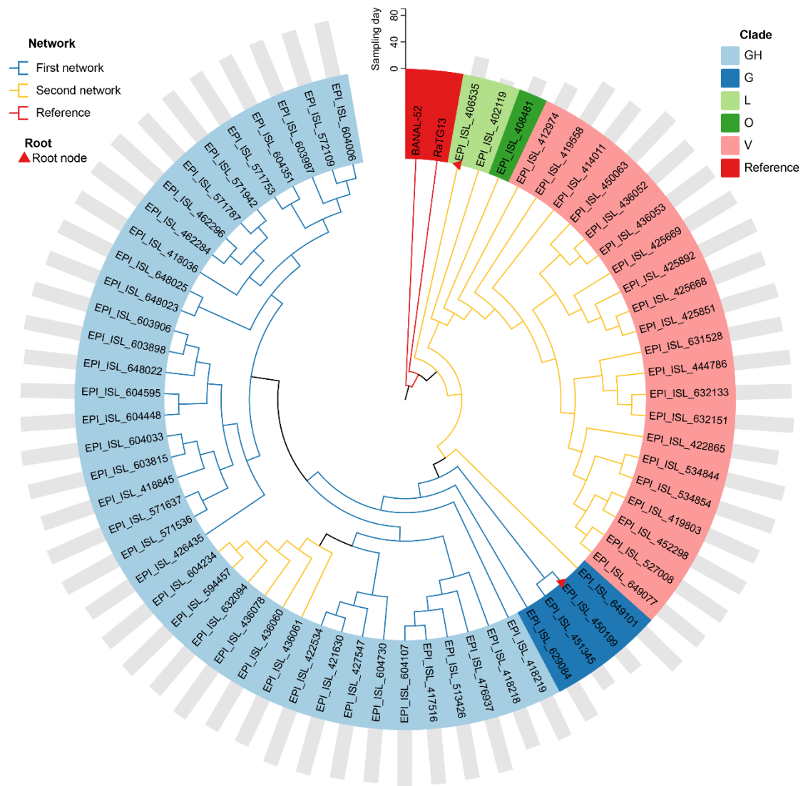
Supplementary Figure S7 Comparison between our approach and maximum-likelihood phylogenetic tree using node samples from two transmission networks with longest chain lengths
