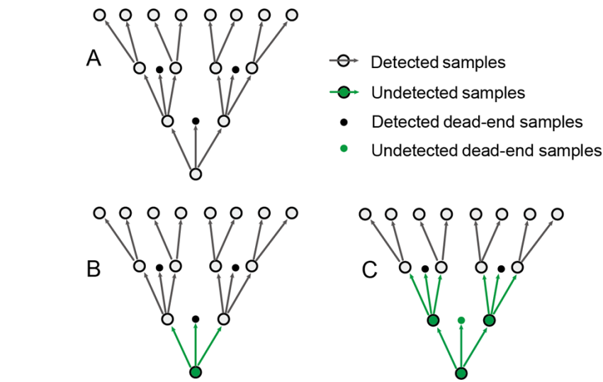
Supplementary Figure S1 Three hypotheses of SARS-CoV-2 transmission network, reconstructed using detected samples
