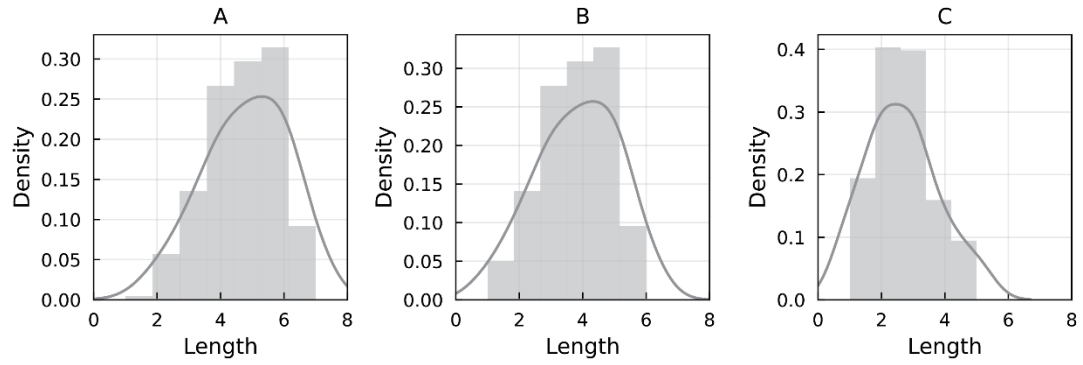
Supplementary Figure S5 Kernel density of transmission chains with different chain lengths using simulation data
