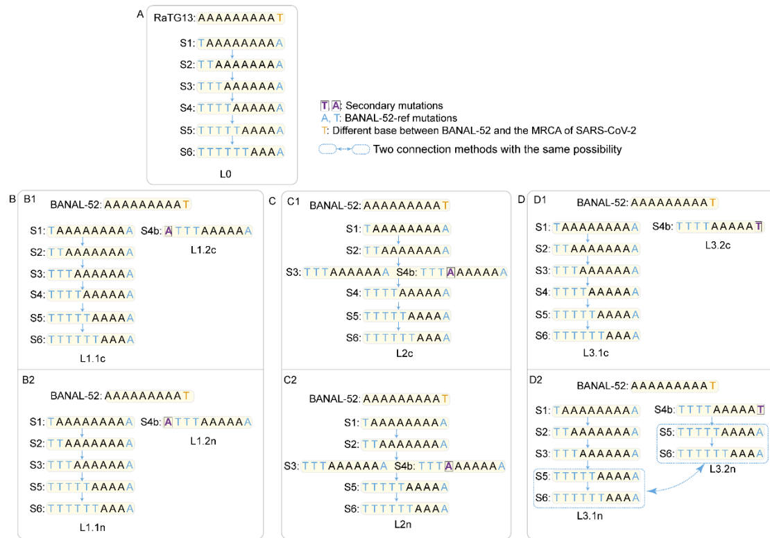
Supplementary Figure S2 Illustration of model errors caused by secondary mutations during three-month study period (i.e., bold purple boxed T or A in sequence S4) in reconstruction of transmission chains and networks using BANAL-52 as a reference
