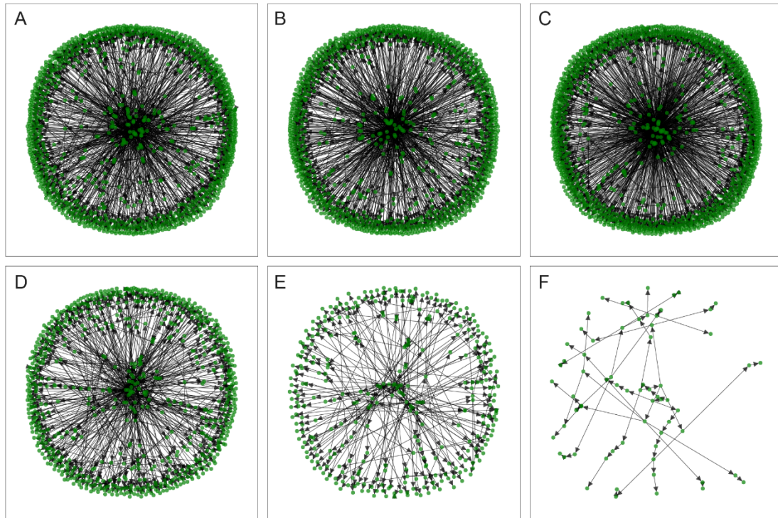
Supplementary Figure S4 Reconstructed transmission networks of SARS-CoV-2 with four nodes (A), five nodes (B), six nodes (C), seven nodes (D), eight nodes (E), and nine nodes (F) using BANAL-52-referenced mutations
